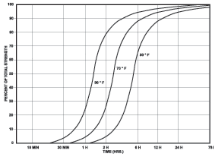
Graph V: Rate of cure at various temperatures
