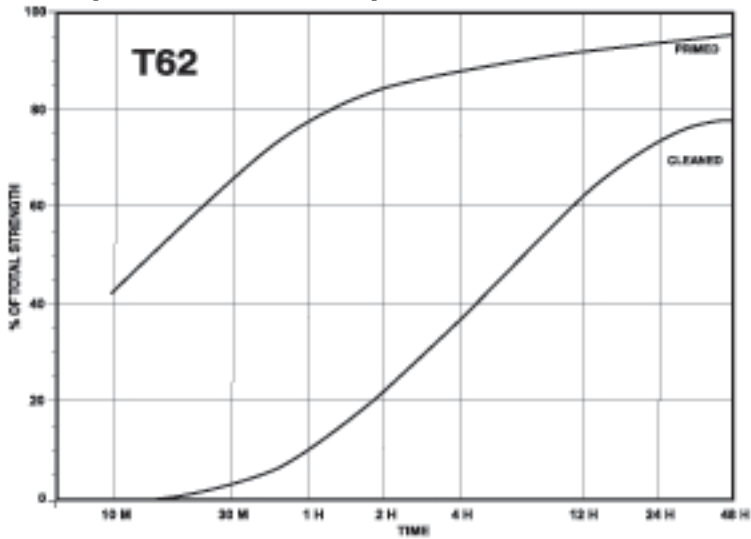
Graph III: Rate of cure on Zinc plated 3/8 x 16 UNC fasteners
